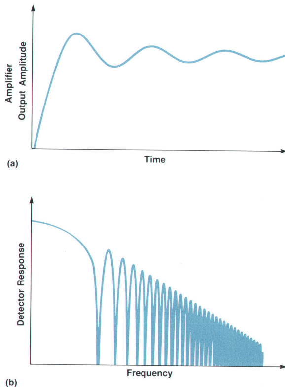
Fig. 10. Integrating detector measurement system characteristics. (a) Damped oscillation output of amplifier. (b) Response of integrating analog-to-digital detector versus frequency.
