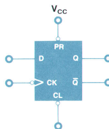
Fig. 5. (a) D-type flip-flop and library test sequence. (b) Use of flip-flop on board under test. For this topology, the library test is modified by removing test vector unit one.
