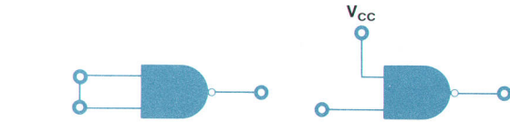
Fig. 2. Configurations of a NAND gate used as an inverter.
